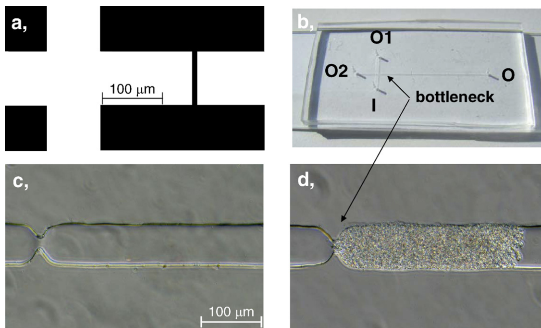
Fig. 2. (a) Part of the lithographic mask pattern about the crossing of channels and the 4 \mu\text{m} wide line positioned close to the crossing to create a bottleneck in the chip (starting point to retain particles in the channel). (b) Photo of the microchip (I: sample inlet, O: separation outlet, O1 and O2 are outlet reservoirs). The suspension of particles is pumped from O during the packing, the sample solutions to be separated or preconcentrated are injected from I). Optical micrographs of the fluid channel with the frit-like bottleneck (c) and the created packing of ground silica aerogel particles (particles were pumped from O port (d)).
